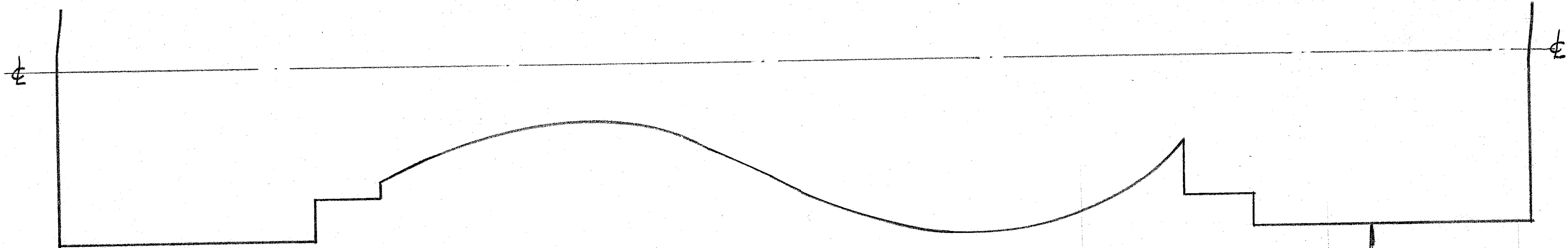
DETAIL OF BACK BALUSTRADE - PROFILE (FULL SIZE)
